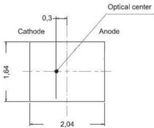
Chip position Top view
