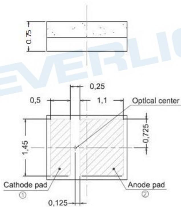
Bottom view
